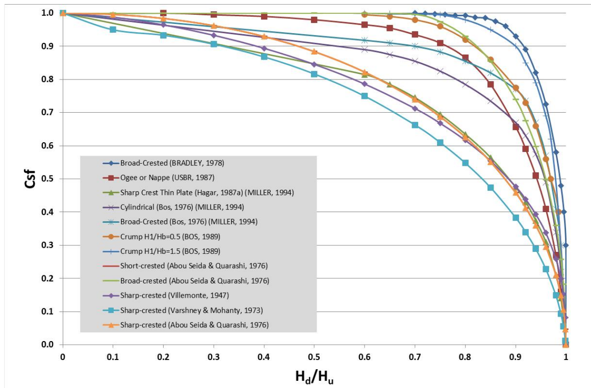
Figure 5-4 Weir Submergence Curves from the Literature
