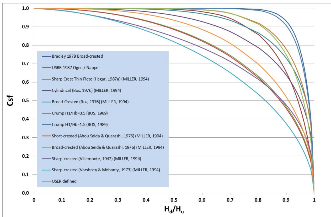
Figure 5-5 Weir Submergence Curves using Villemonete Equation
