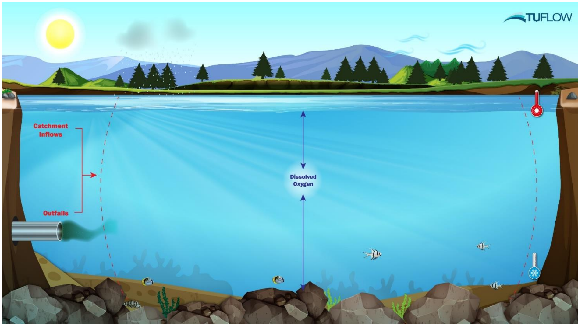
Figure 2-2 Conceptual diagram: DO Simulation Class
