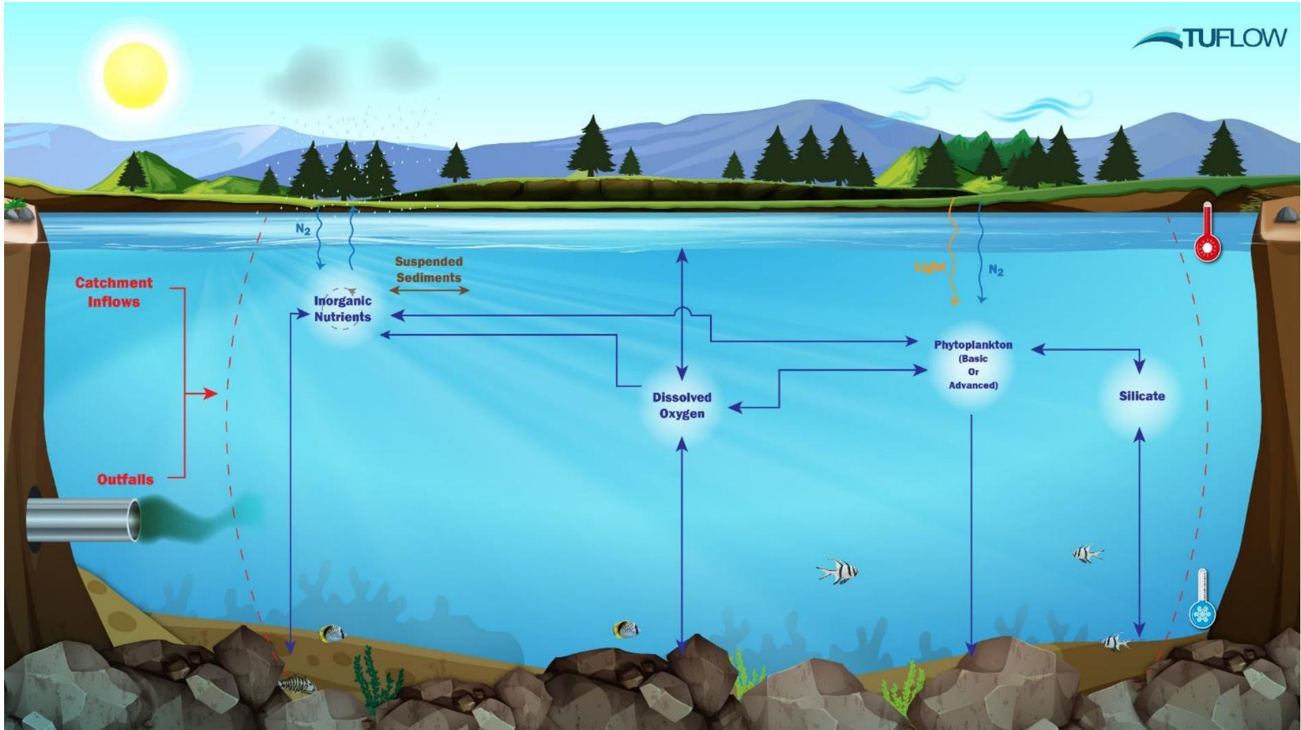
Figure 2-3 Conceptual diagram: Inorganics Simulation Class
