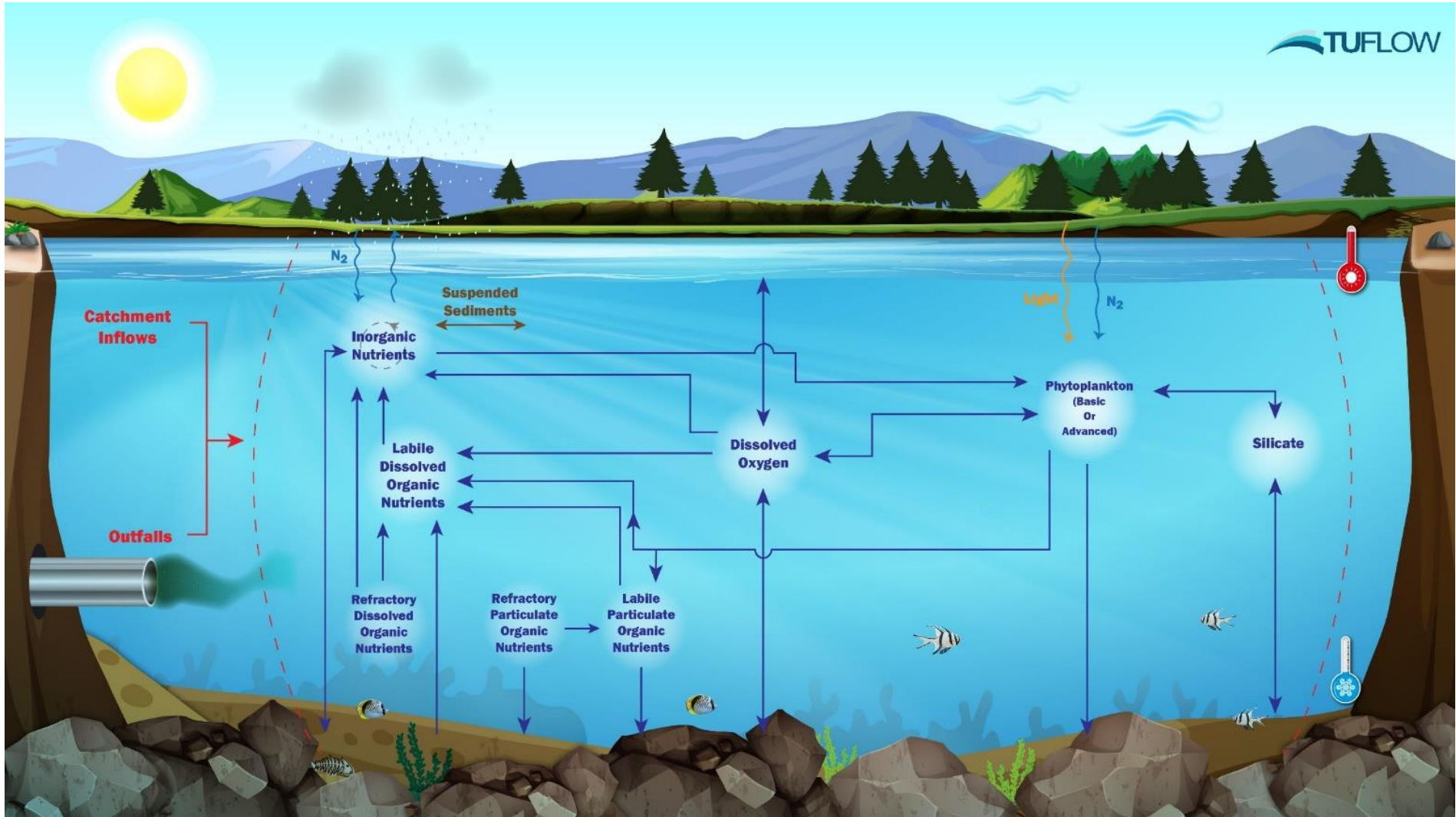
Figure 2-4 Conceptual diagram: Organics Simulation Class
