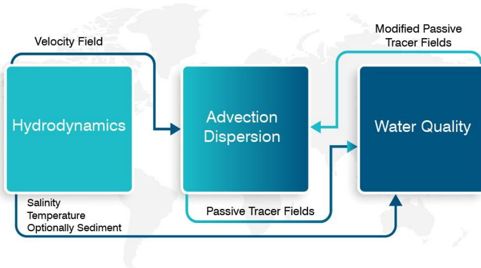
Figure 2-1 Interaction of TUFLOW FV's HD engine, AD and WQ Modules
