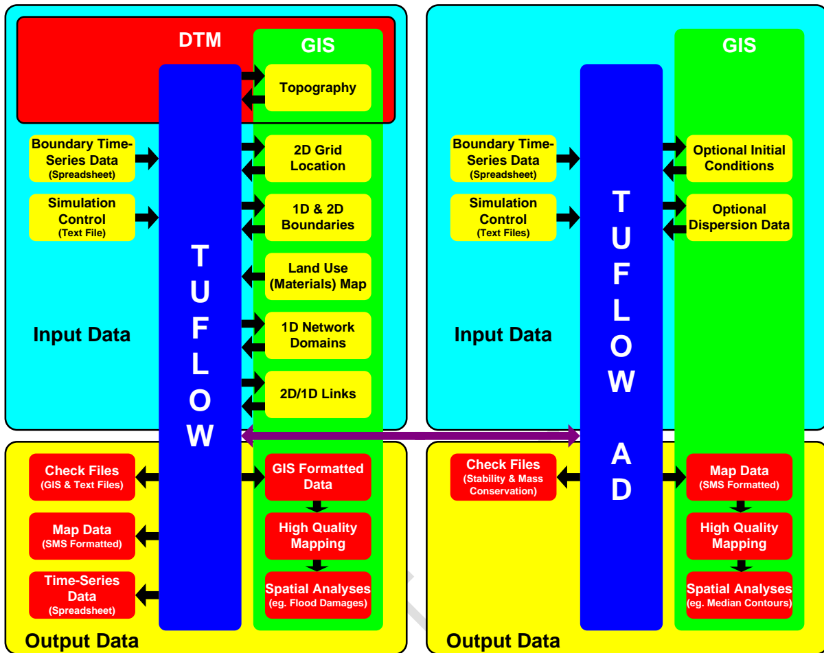
Figure 2-1 TUFLOW and TUFLOW AD Relationship and Data Input and Output Structure
