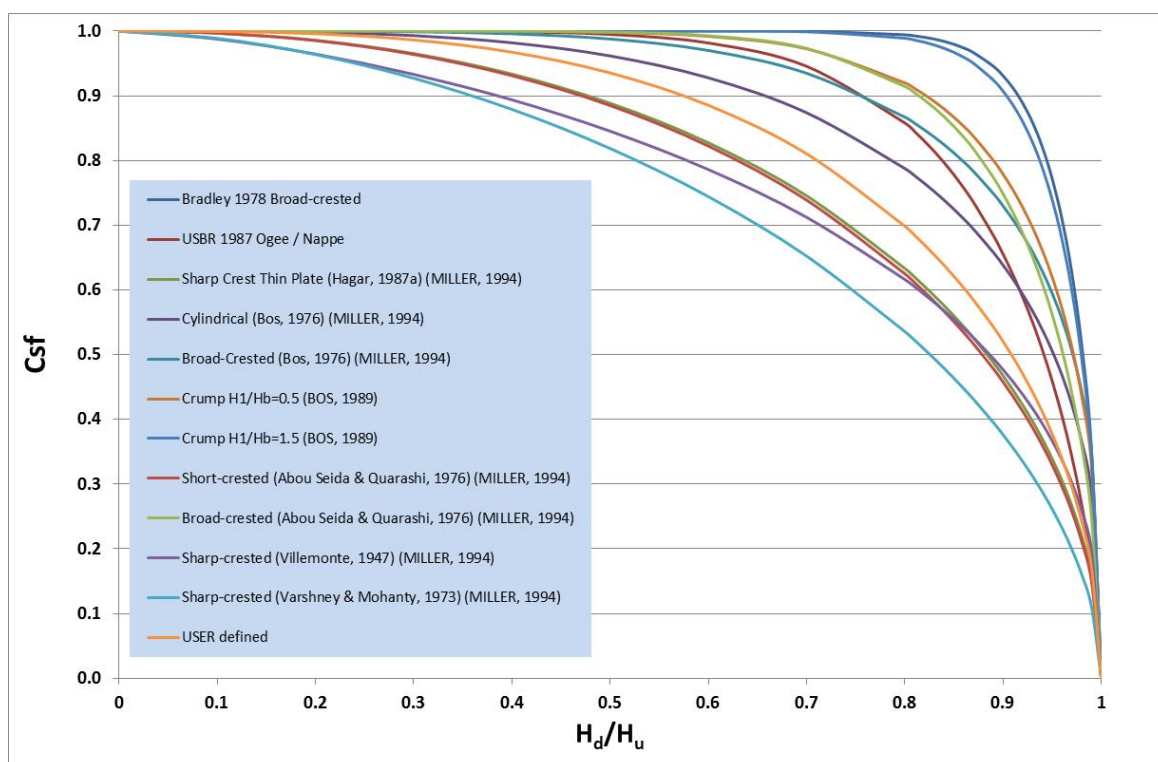
Figure 5-5 Weir Submergence Curves using Villemonthe Equation
